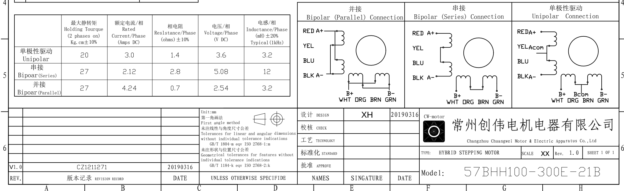
3 WIRINGS CONNECTION DIAGRAM
