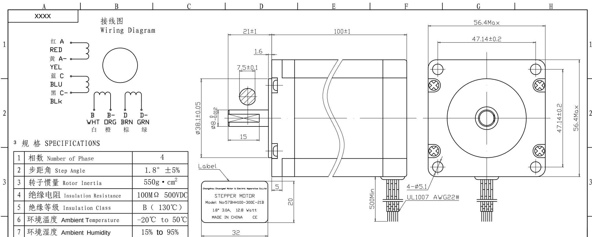
3 WIRINGS CONNECTION DIAGRAM
